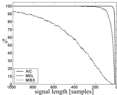
Fig. 1. Accuracy of the dimension estimation by AIC, MDL and MIBS depending on the signal length.
