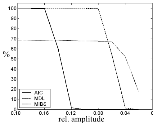
Fig. 2. Accuracy of the dimension estimation by AIC, MDL and MIBS depending on the relative amplitude of two sinusoidal components.
