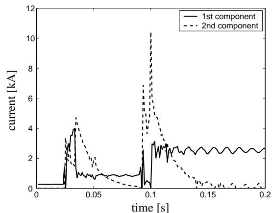
Fig. 8. Time-varying amplitude of the two components of the current.
