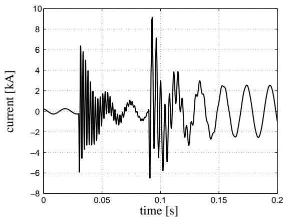
Fig. 6. Waveform of the A-phase current during switching of the condenser banks in the transmission line.
