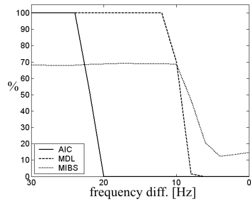
Fig. 3. Accuracy of the dimension estimation by AIC, MDL and MIBS depending on the difference of frequencies of two sinusoids with equal amplitude.
