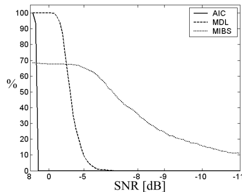
Fig. 4. Accuracy of the dimension estimation by AIC, MDL and MIBS depending on the Signal-to-Noise Ratio.
