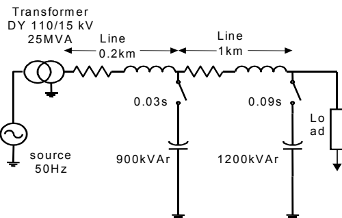
Fig. 1 One-phase diagram of the simulated system.
