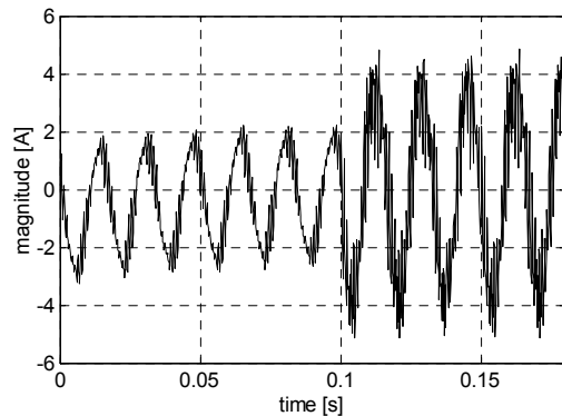
Fig. 10. Current waveform at the inverter output.
