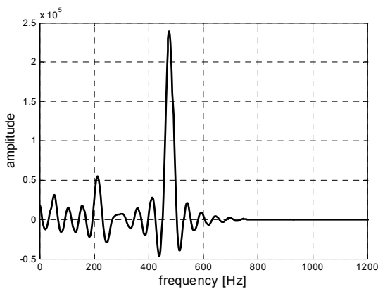
Fig. 7. Cross-section of the time-frequency representation from Fig. 6 for the time t=0.04 s.
