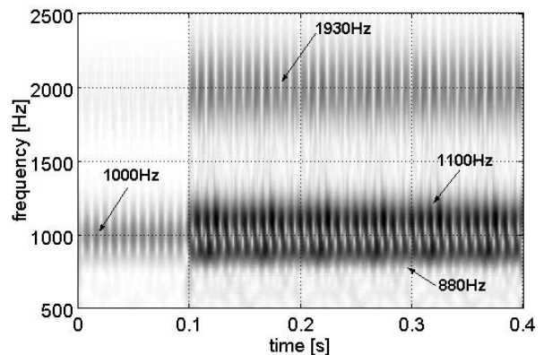
Fig. 11. Time frequency representation of the signal taken from the fault operation of the inverter drive, obtained using the Complex Morlet Wavelet, f_b=1 ; f_c=1 , scale=0.1:0.1:10.
