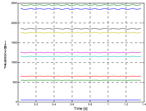
Figure 5: ESPRIT representation of the MV voltage at the DC arc furnace without compensation. Analysis window of 300 samples (sampling frequency 5000 Hz).
