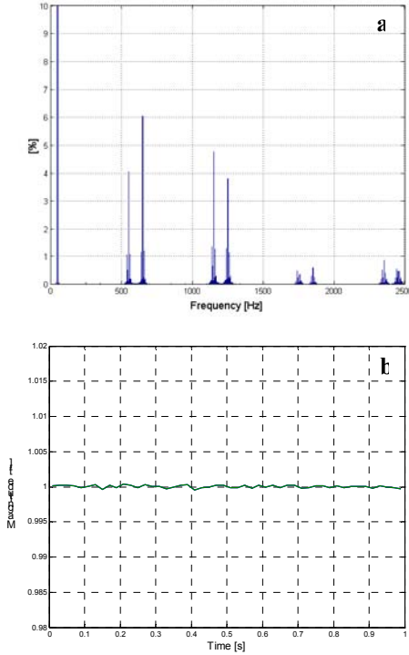
Figure 3: Voltage at the DC arc furnace with STATCOM: a) spectrum (FFT on 1 s window); b) fundamental component's magnitude versus time (PRONY representation for 100 samples in window analysis, sampling frequency 5000 Hz)
