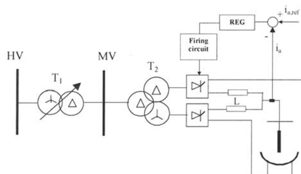
Figure 1: Modelled dc arc furnace plant.
