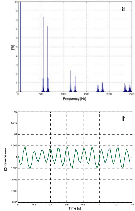
Figure 2: Voltage at the DC arc furnace without compensation: a) spectrum (FFT on 1 s window); b) fundamental component's magnitude versus time (PRONY representation for 100 samples in window analysis, sampling frequency 5000 Hz).
