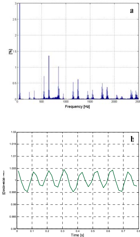
Figure 4: Voltage at the DC arc furnace with Active Filter: a) spectrum (FFT on 1 s window); b) fundamental component's magnitude versus time (PRONY representation for 100 samples in window analysis, sampling frequency 5000 Hz)
