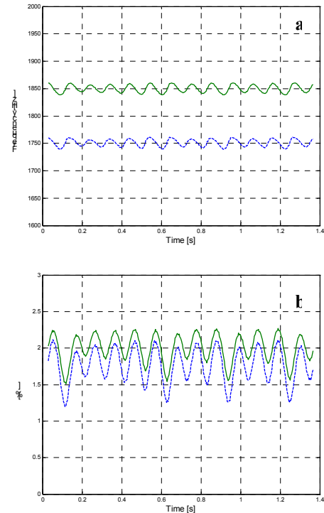
Figure 7: Time-varying frequency (a) and relative amplitude (b) (relative to the mean amplitude over the analysis interval) of MV voltage without compensation at the 1600-2000 Hz band.
