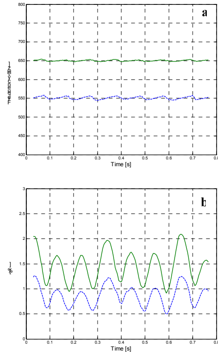
Figure 6: Time-varying frequency (a) and relative amplitude (b) (relative to the mean amplitude over the analysis interval) of MV voltage with active filters at 11 th and 13 th harmonic.
