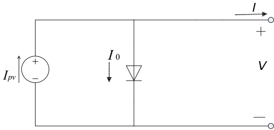
Fig. 1 Ideal Single Diode Model (ISDM)
